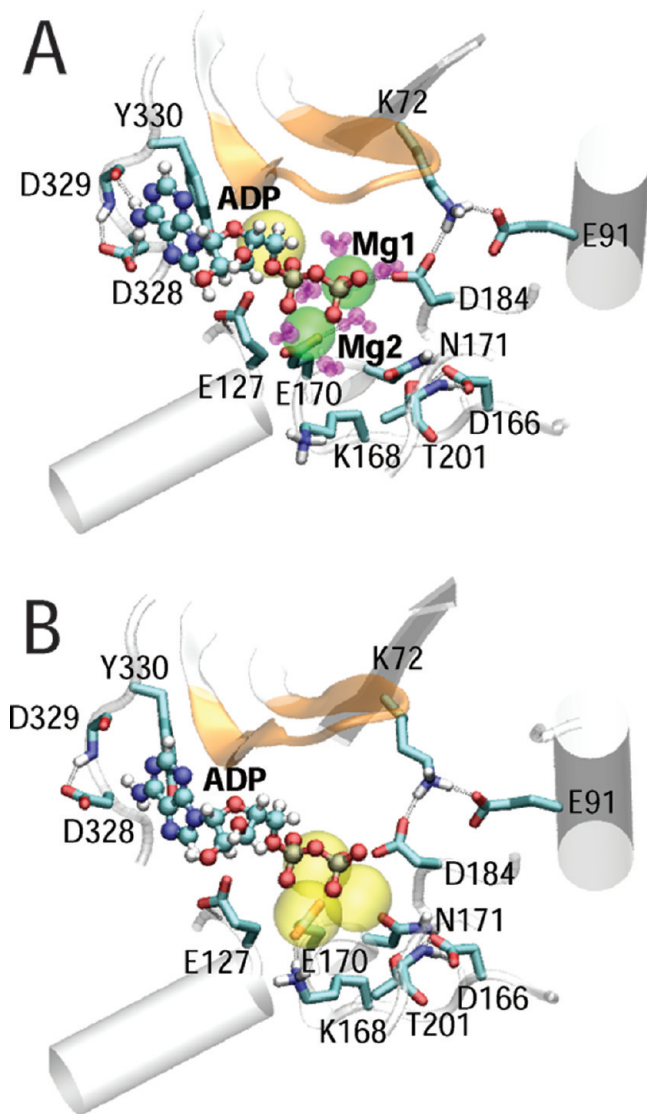
FIGURE 6: A snapshot from an optimized intermediate state ensemble: the active site of the PKA during ADP release with (A) and without (B) \text{Mg}^{2+} ions. The Gly-rich loop is shown in cartoon representation in transparent orange color. All the other secondary structure elements of the protein frame that are relevant to the active site are shown in transparent white-gray. The ADP is shown with ball-and-stick model. The important active site residues are depicted in licorice representation. The \text{Mg}^{2+} and \text{Na}^{+} ions are shown in green and yellow transparent balls, respectively. Water molecules coordinating \text{Mg}^{2+} ions are shown in transparent pink color. Some of the hydrogen bonds present are depicted with dashed bonds.
